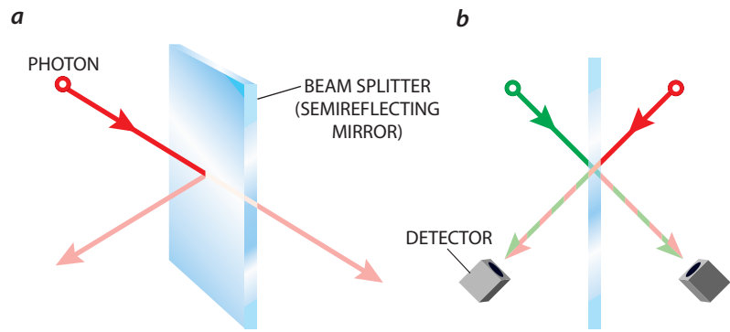
BEAM SPLITTER , or semireflecting mirror (a), reflects half the light that hits it and transmits the other half. An individual photon has a 50–50 chance of reflection or transmission. If two identical photons strike the beam splitter at the same time, one from each side (b), the reflected and transmitted parts interfere, and the photons lose their individual identities. We will detect one photon in each detector 25 percent of the time, and it is then impossible to say if both photons were reflected or both were transmitted. Only the relative property—that they went to different detectors—is measured.
